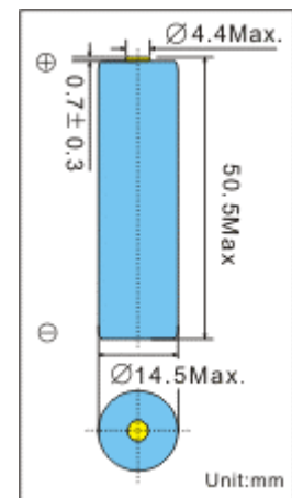
UNTAGGED BATTERY DIMENSIONS
